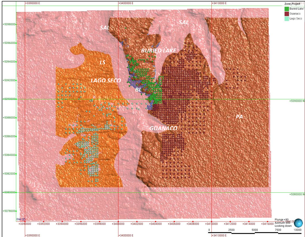
Figure 14-1. Plan view of the Laguna Salada Project showing the surface control, sample locations and interpreted mineralization model extents for the Pampa de Arroqui Formation (PA – copper), Laguna Salada Formation (LS – orange), Buried Lake Formation (BL – dark blue), and Salamanca Formation (SAL – pink); see Figure 14-2 (Atticus, 2026).
