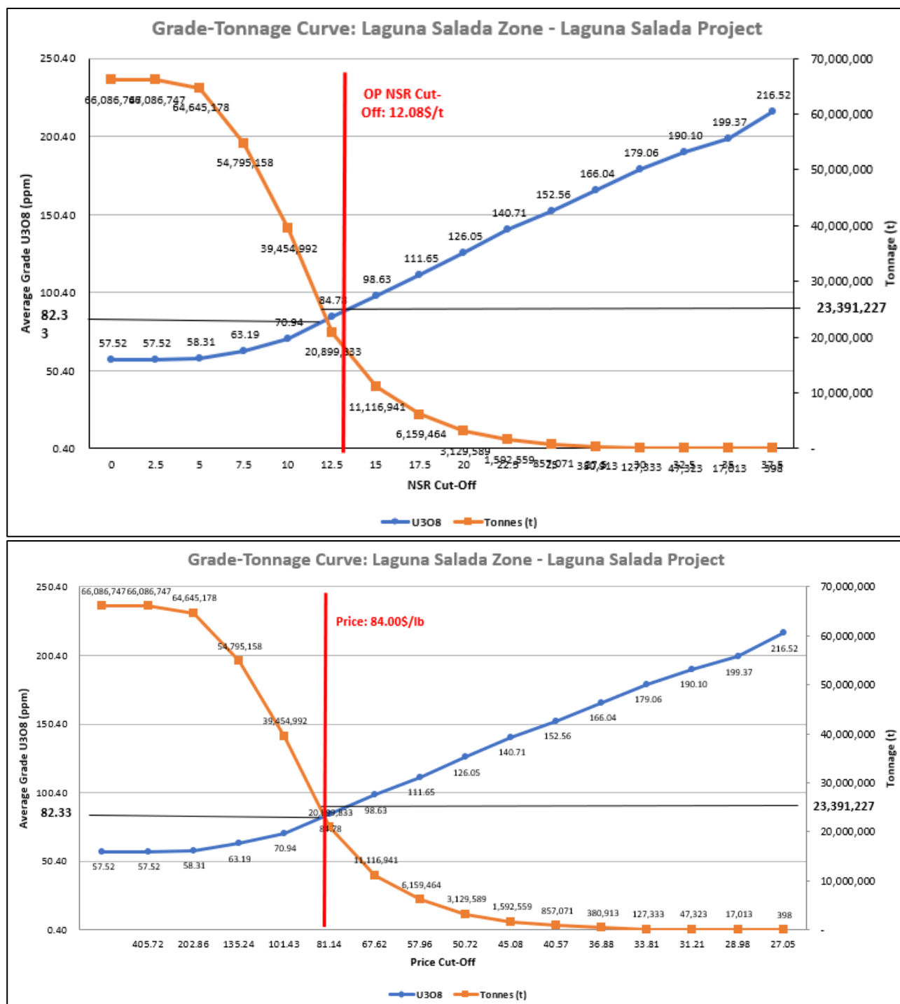
Figure 14-38. Laguna Salada grade-tonnage sensitivity curves showing tonnes and average U 3 O 8 grade by NSR cut-off in the upper panel, with the selected US$12.08/t reporting cut-off highlighted, and by equivalent U 3 O 8 price in the lower panel, with the selected US$84/lb reference price highlighted (Atticus, 2026).
