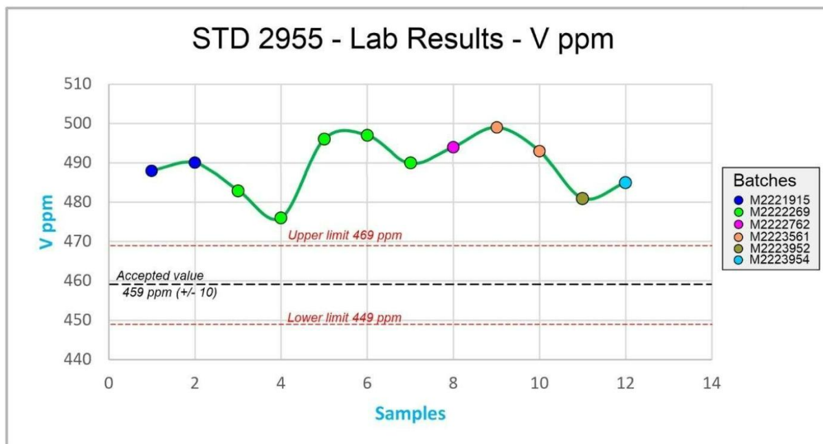
Figure 11-6. Vanadium values for standard STD 2955 (Miller, 2024).
