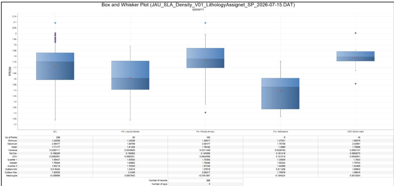
Figure 14-21. Box and whisker plot of average bulk-density measurements by assigned lithological unit (Atticus, 2026).
