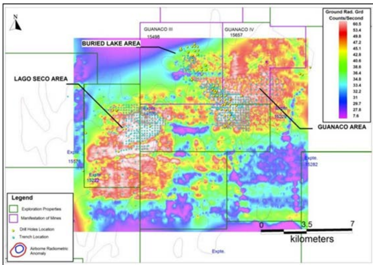
Figure 6-2. Radiometric anomalies and trenching at Laguna Salada (after Inwood and Goode, 2011) (Miller, 2024).
