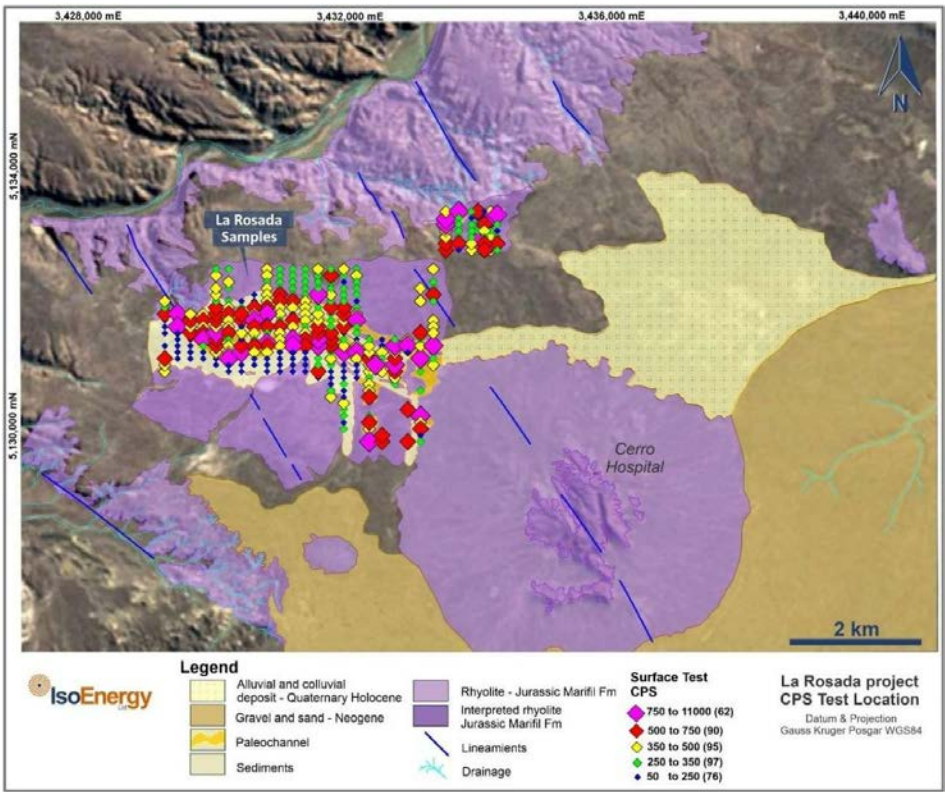
Figure 11-9. Scintillometer (cps) measurements at the La Rosada area (Miller, 2024).
