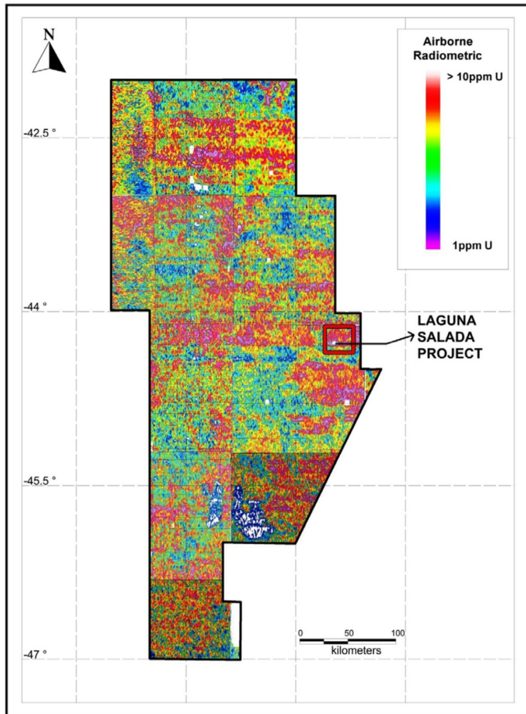
Figure 6-1. Map showing the extent of the CNEA radiometric survey that covers part of the Laguna Salada Project (Tenova, 2014).
