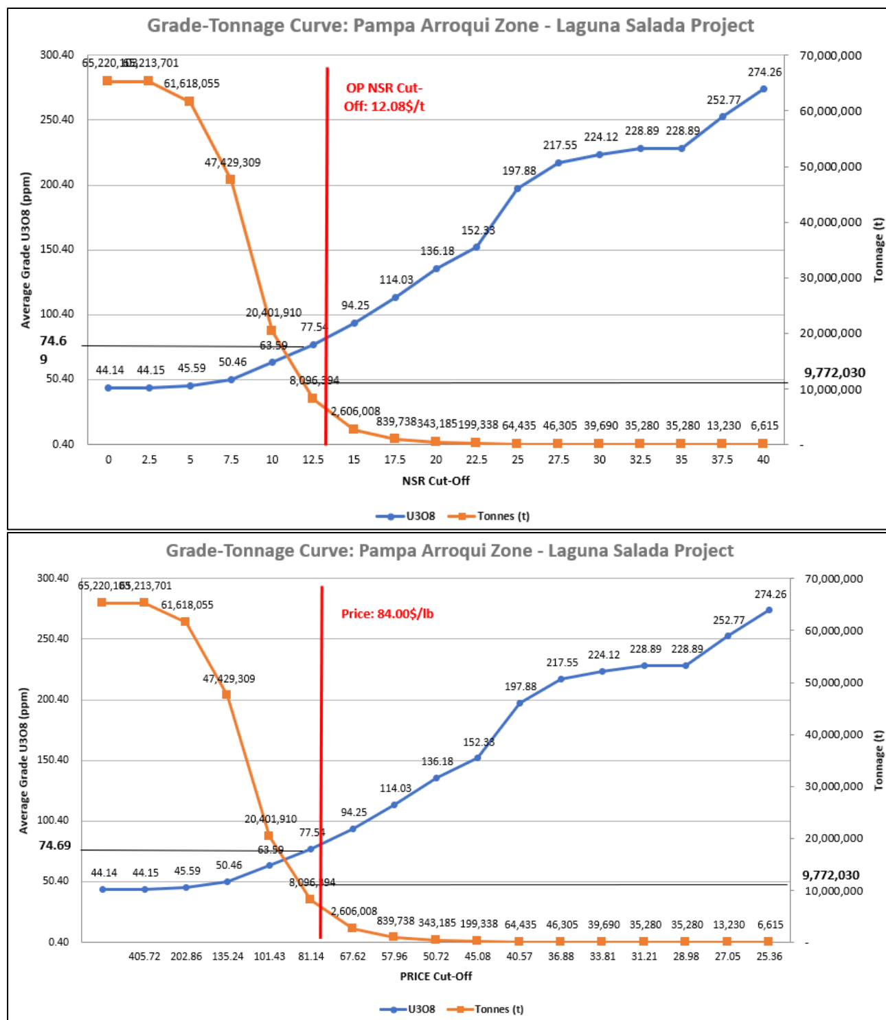
Figure 14-40. Pampa de Arroqui grade-tonnage sensitivity curves showing tonnes and average U 3 O 8 grade by NSR cut-off in the upper panel, with the selected US$12.08/t reporting cut-off highlighted, and by equivalent U 3 O 8 price in the lower panel, with the selected US$84/lb reference price highlighted (Atticus, 2026).
