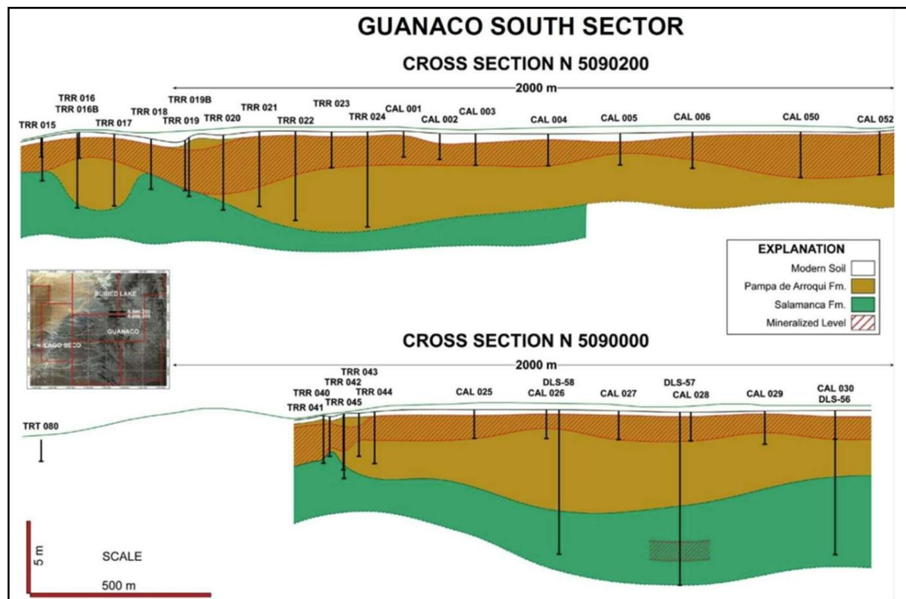
Figure 7-6. Geology and mineralization at the Guanaco area. Note extreme vertical exaggeration (after Inwood and Goode, 2011) (Miller, 2024).
