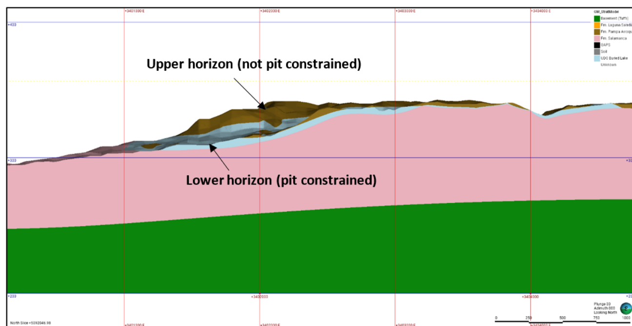
Figure 14-44. Detailed cross-section through the Guanaco–Buried Lake area showing the relationship between the upper, not pit constrained Pampa de Arroqui mineralized horizon and the lower, pit constrained Buried Lake mineralized horizon near the Pampa de Arroqui–Salamanca Formation contact. The section is displayed with 10× vertical exaggeration (Z-scale = 10.0) for visualization (Atticus, 2026).
