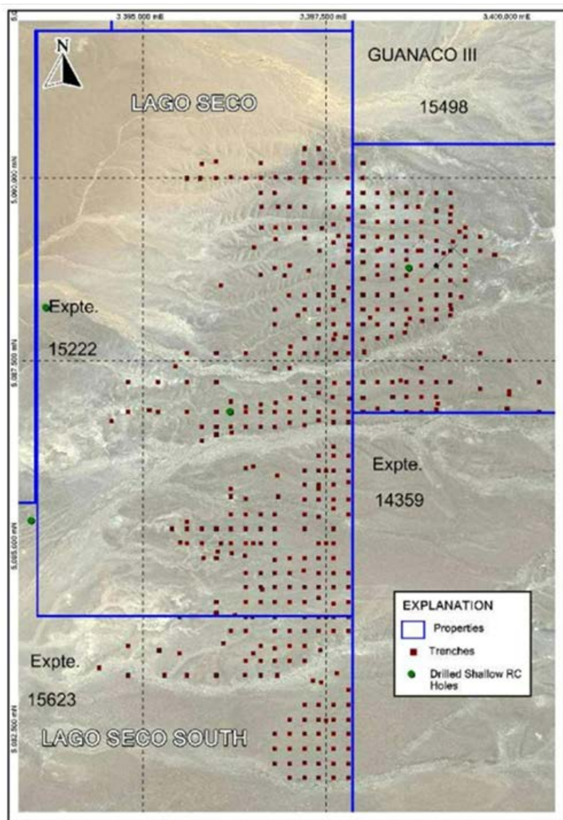
Figure 6-7. Map showing the location of trenches and drill hole collars in the Lago Seco area (after Inwood and Goode, 2011) (Miller, 2024).
