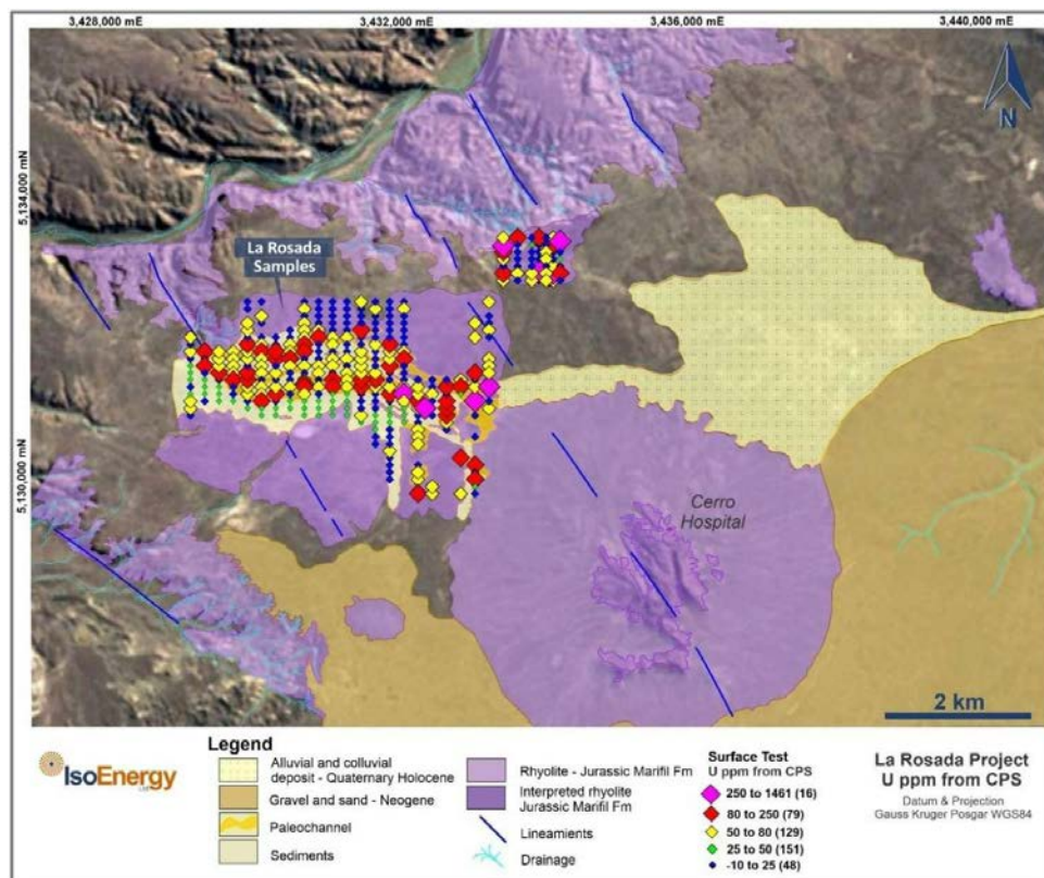
Figure 11-10. Predicted uranium values in ppm based on scintillometer readings at the La Rosada Area (Miller, 2024).
