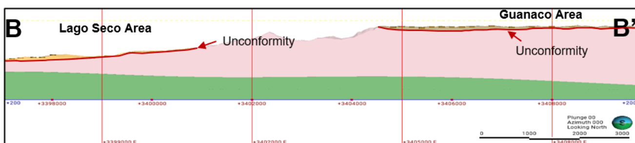
Figure 14-5. Interpreted lithological section B-B' through the Laguna Salada model, showing the stratigraphic relationship between the Lago Seco and Guanaco areas and the interpreted unconformity surfaces at or near the top of the conglomeratic units. The section is displayed with 10× vertical exaggeration (Z-scale = 10.0) for visualization (Atticus, 2026).
