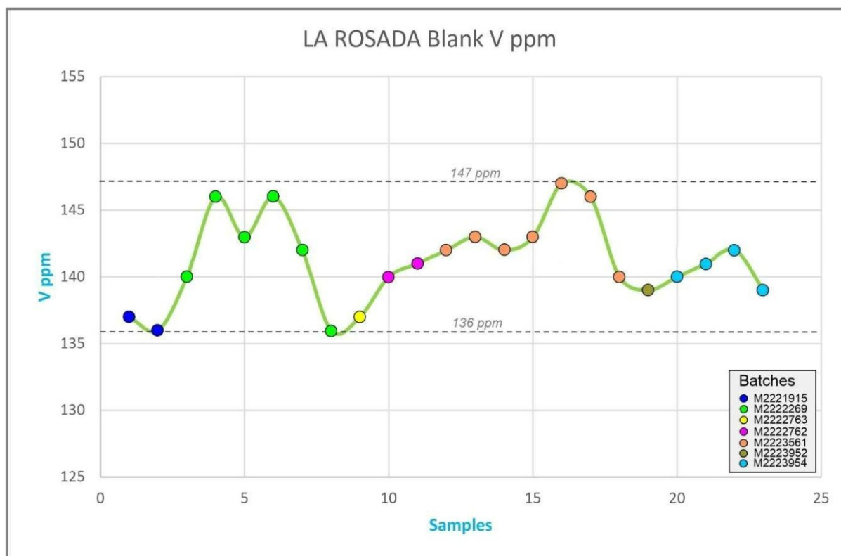
Figure 11-4. Vanadium values for blank material showing batch numbers (Miller, 2024).
