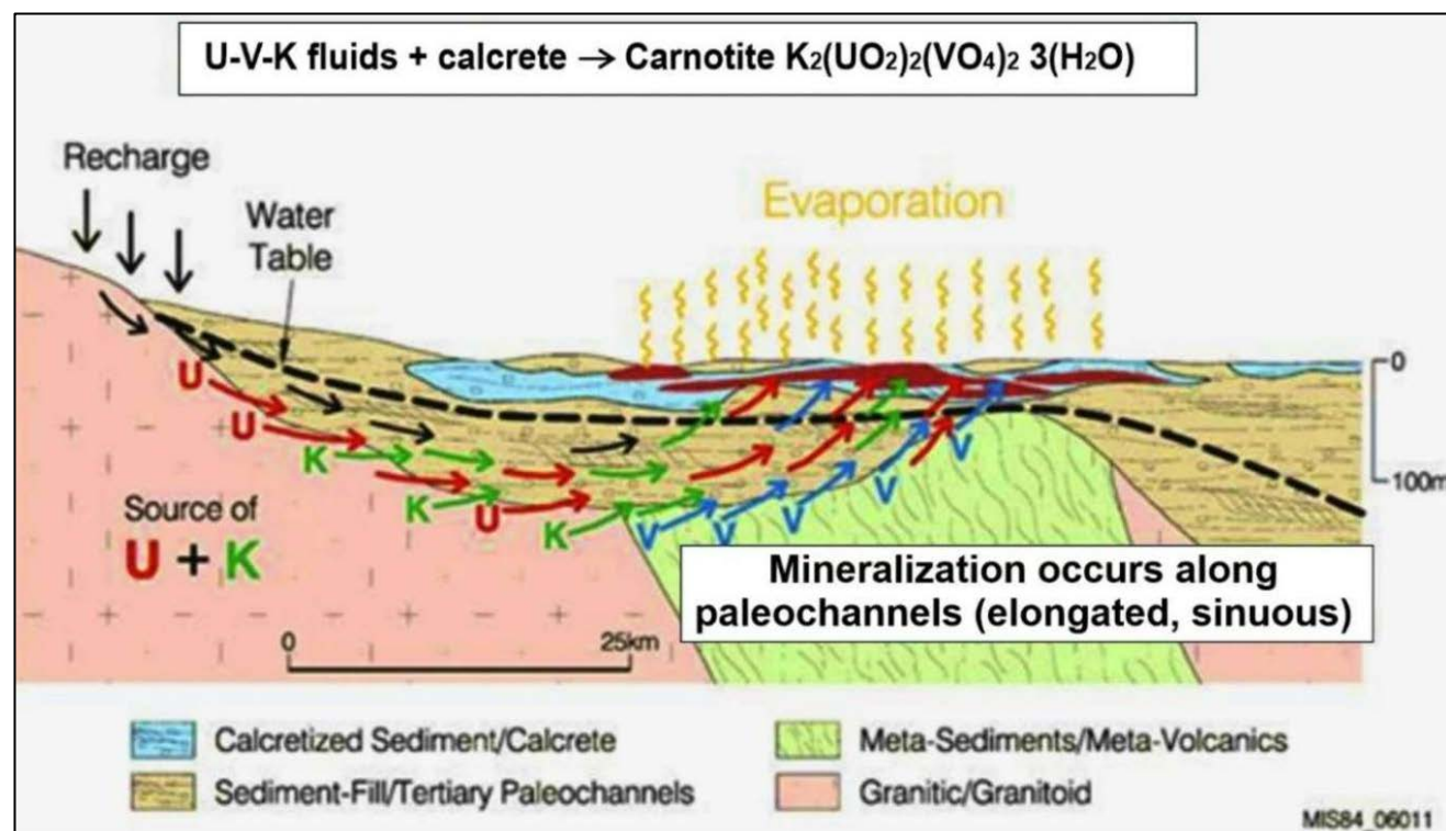
Figure 8-1. Genetic model for the formation of surficial uranium deposits (Miller, 2024).
