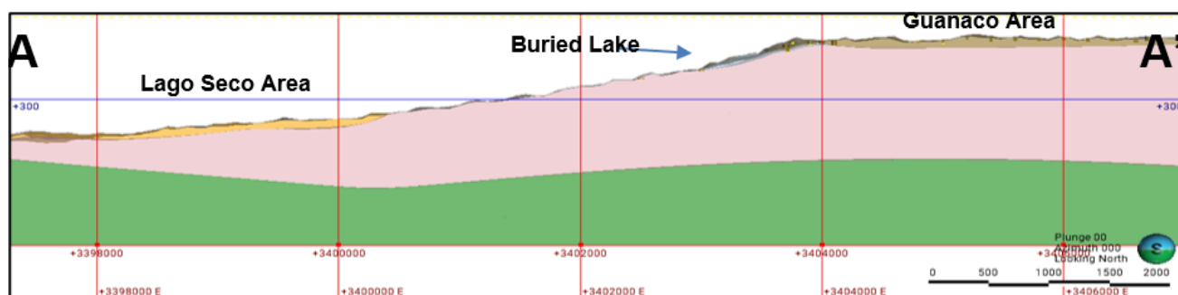
Figure 14-4. Interpreted lithological section A-A' through the Laguna Salada model, showing the relationship between the Lago Seco and Guanaco areas and the position of the Buried Lake unit near the Pampa de Arroqui Formation to Salamanca Formation contact. The section is displayed with 10× vertical exaggeration (Z-scale = 10.0) for visualization (Atticus, 2026).
