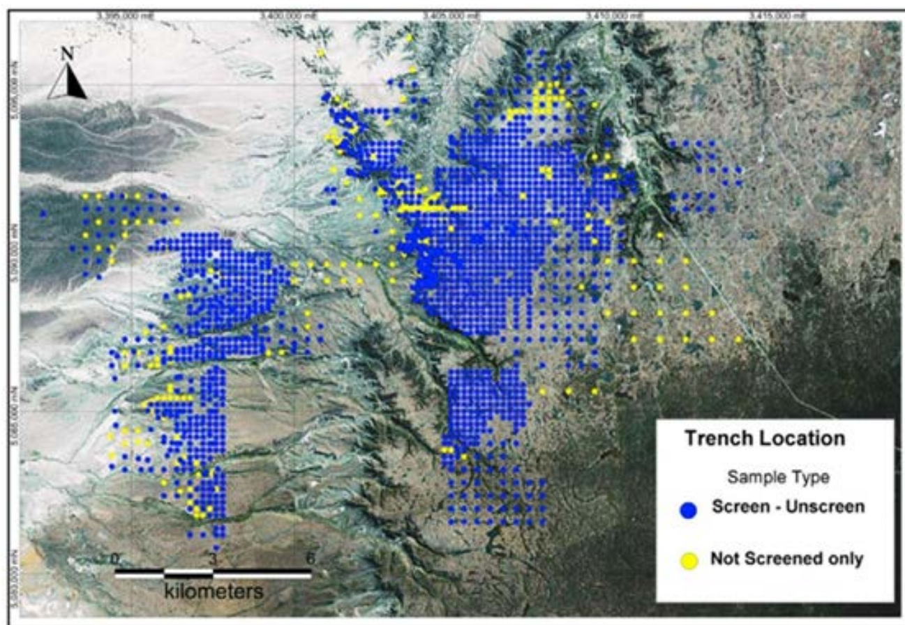
Figure 11-1. Plan map showing the location of the trenches and pits at Laguna Salada, coloured according to the sampling method used (after Tenova, 2014) (Miller, 2024).
