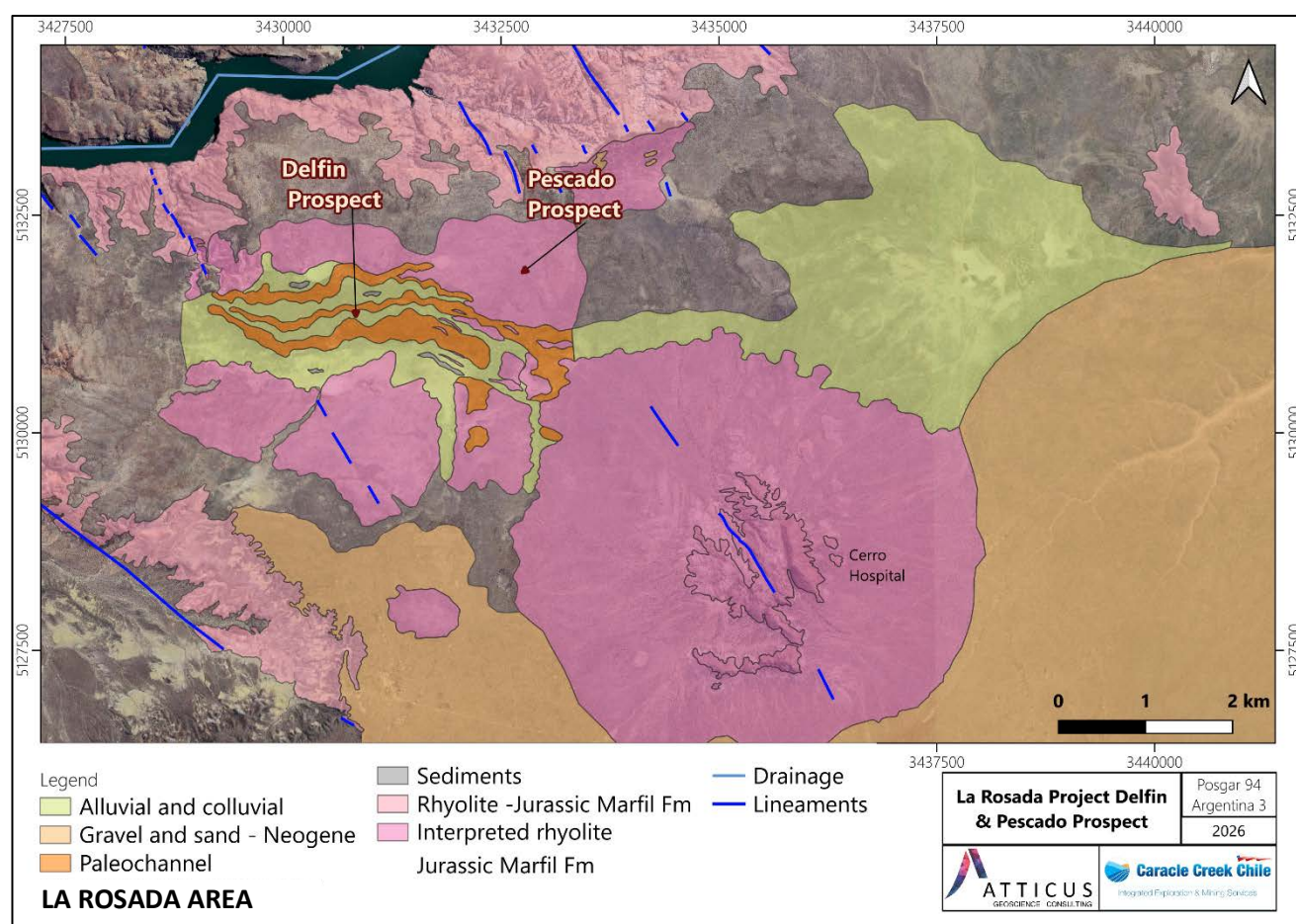
Figure 6-17. Local geology around the Delfin and Pescado prospects at the La Rosada area (Miller, 2024).
