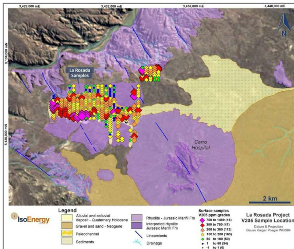
Figure 11-11. Vanadium concentrations and geology at the La Rosada area (Miller, 2024).
