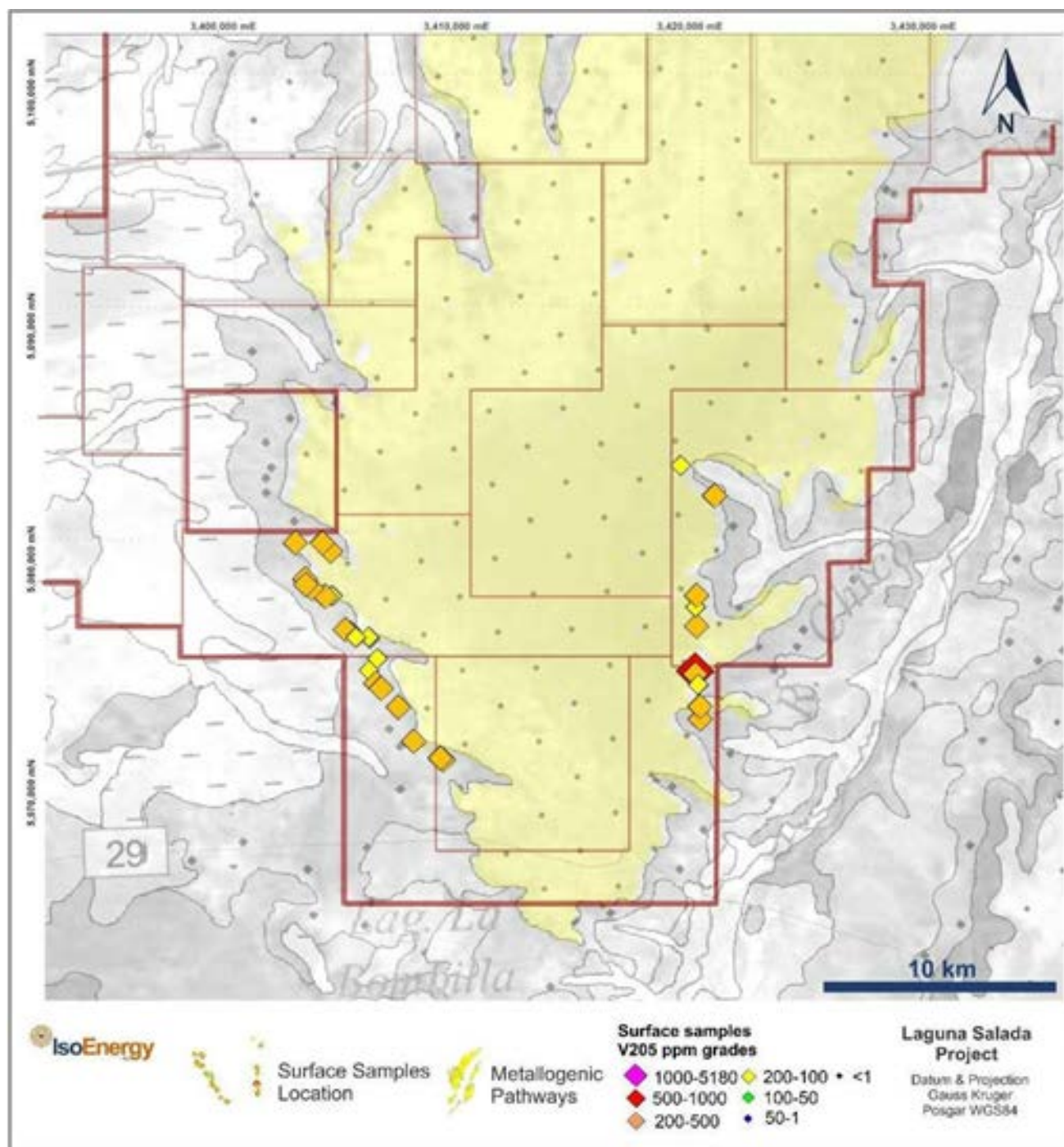
Figure 6-14. La Susana area of the Laguna Salada Property (historical boundary) showing surface sample locations and V2O5 ppm concentrations (Miller, 2024).
