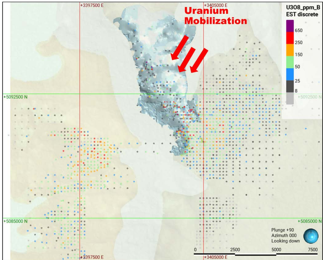
Figure 14-9. Plan view of the Buried Lake mineralization model showing U_3O_8 grade distribution across the interpreted Buried Lake unit and adjacent Pampa de Arroqui area (Atticus, 2026).
