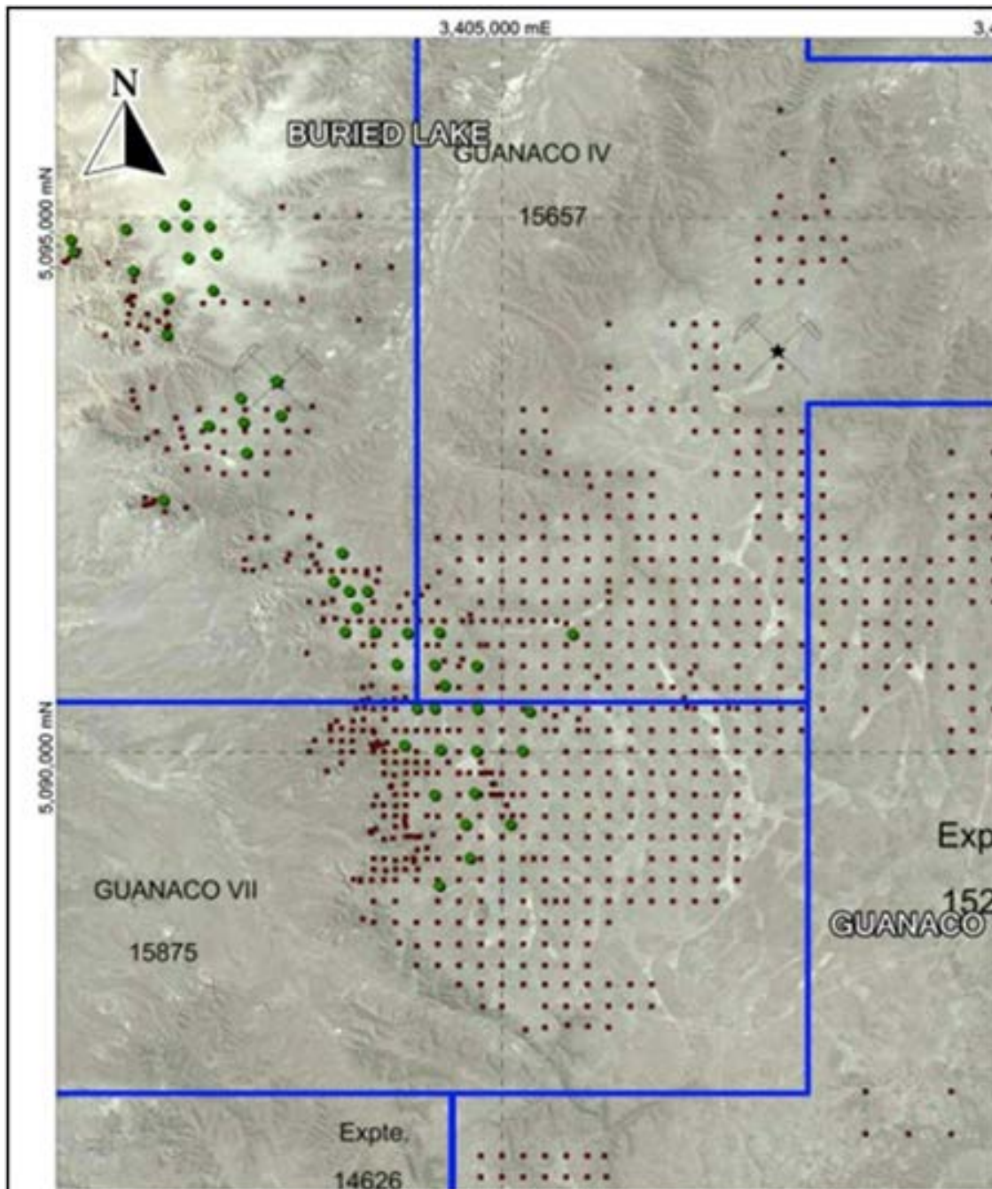
Figure 6-10. Map showing the location of trenches and drill hole collars in the Buried Lake area of the Laguna Salada Project. (after Inwood and Goode, 2011) (Miller, 2024).
