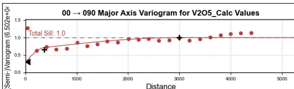
Figure 14-29. Horizontal major-axis variogram for calculated V_2O_5 values in the Pampa de Arroqui estimation domain, showing the fitted model used to support vanadium grade-continuity interpretation (Atticus, 2026).
