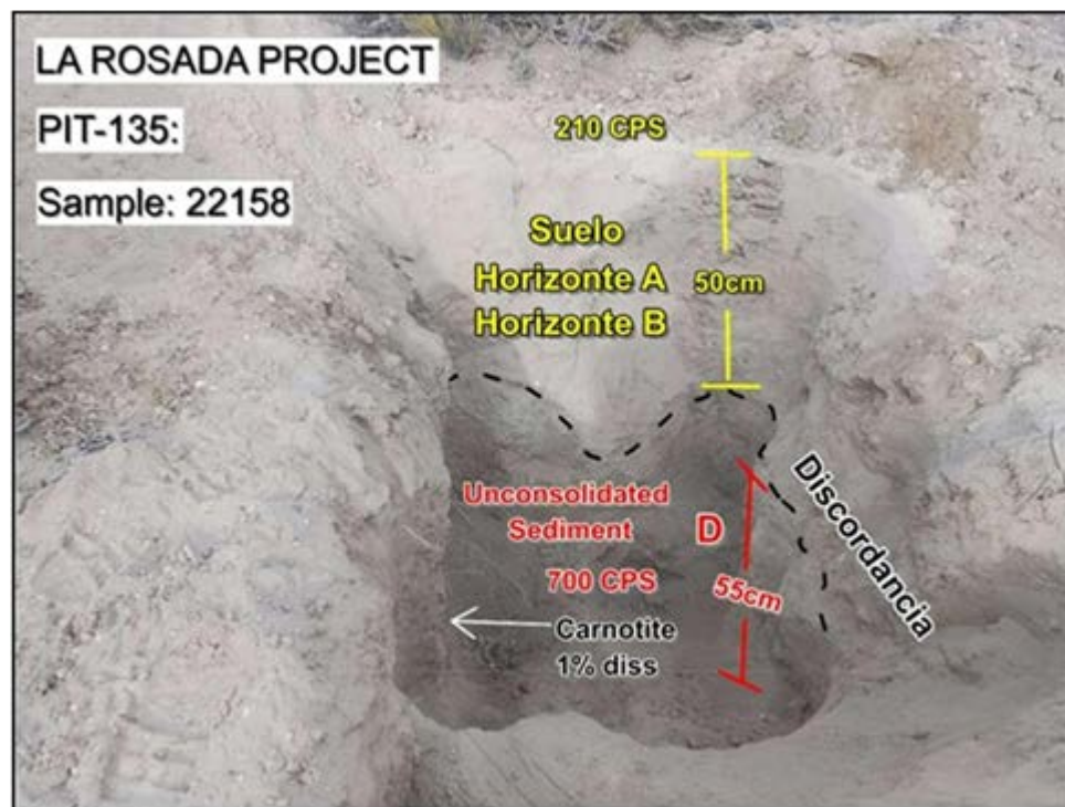
Figure 11-2. Soil profile and Horizon D, unconsolidated sediments (Miller, 2024).
