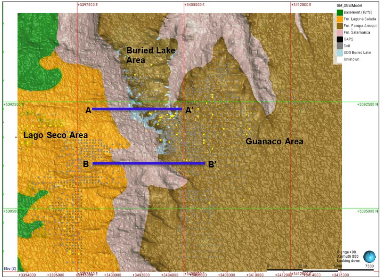
Figure 14-3. Plan view of the Laguna Salada lithology model showing the locations of interpreted section lines A-A' and B-B' across the Lago Seco, Guanaco and Buried Lake areas (Atticus, 2026).
