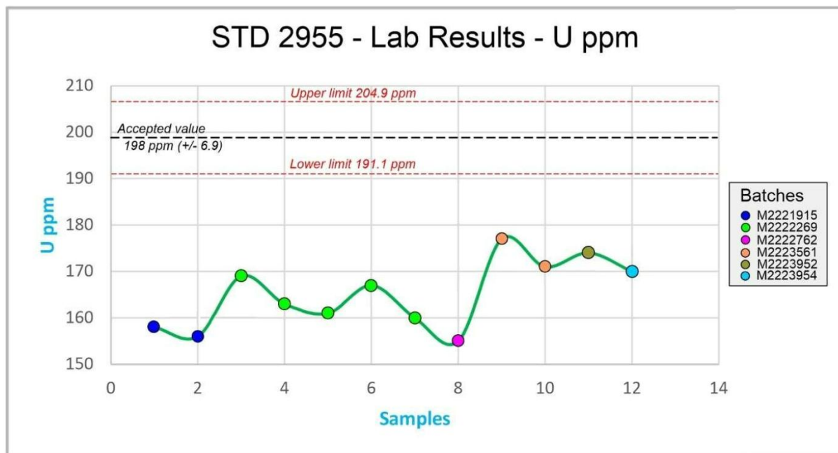
Figure 11-5. Uranium values for standard STD 2955 (Miller, 2024).
