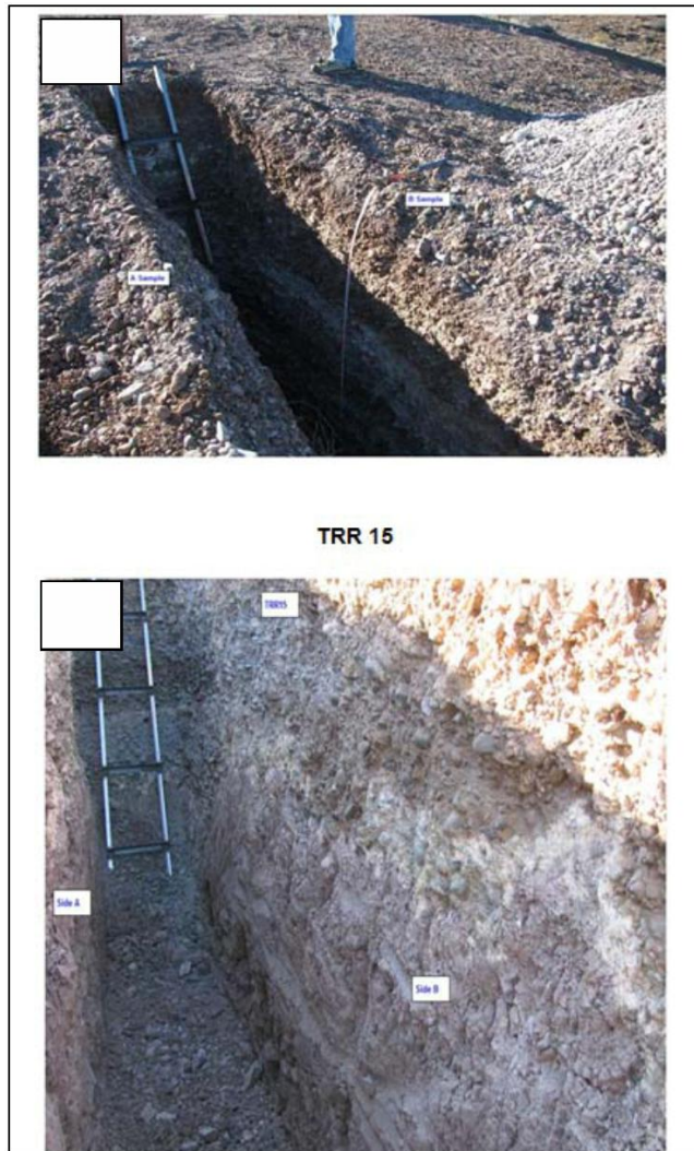
Figure 11-13. Trenches used for independent sampling by Inwood and Goode (2011) (Tenova, 2014).
