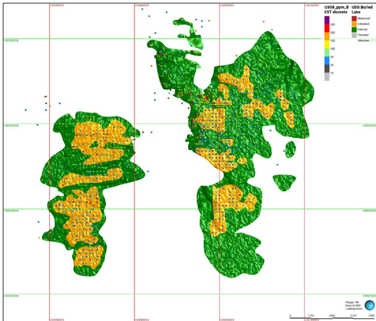
Figure 14-37. Plan view of the Laguna Salada Mineral Resource classification model showing Indicated and Inferred classification across the Laguna Salada, Pampa de Arroqui and Buried Lake estimation domains (Atticus, 2026).
