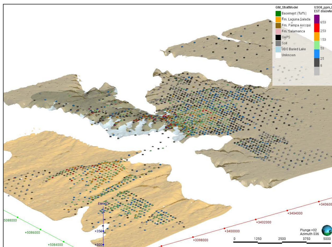
Figure 14-6. Overview of the Laguna Salada mineralization modelling workflow, showing the distribution of U_3O_8 grade points across the Laguna Salada, Pampa de Arroqui and Buried Lake mineralized areas and the use of a 25 ppm U threshold to support mineralization-solid modelling. The view is displayed with 10× vertical exaggeration (Z-scale = 10.0) for visualization (Atticus, 2026).
