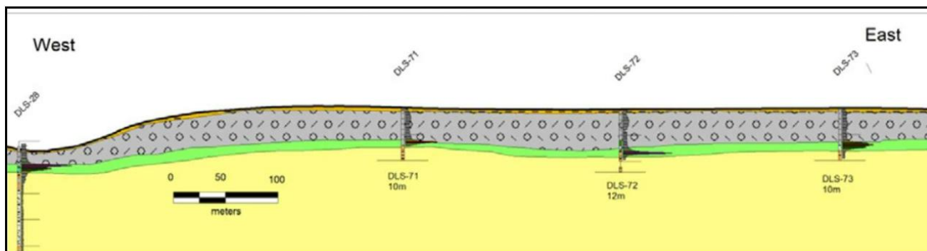
Figure 7-8. Buried Lake schematic cross section showing the lower mineralized horizon (after Inwood and Goode, 2011; Miller, 2024).
