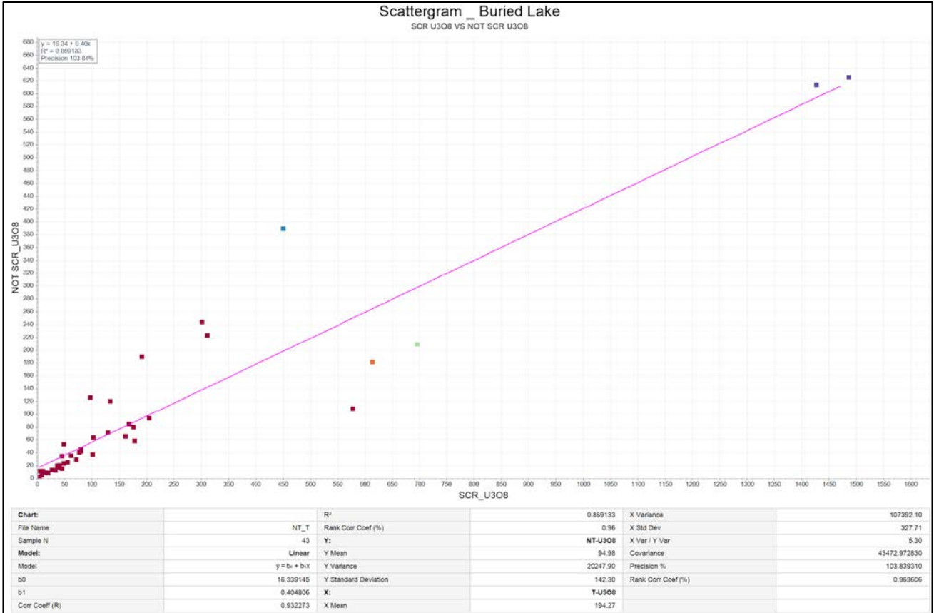
Figure 14-14. Scattergram of screened U 3 O 8 versus unscreened U 3 O 8 for the Buried Lake mineralized area. The x-axis represents U 3 O 8 _T and the y-axis represents U 3 O 8 _NT (Atticus, 2026).
