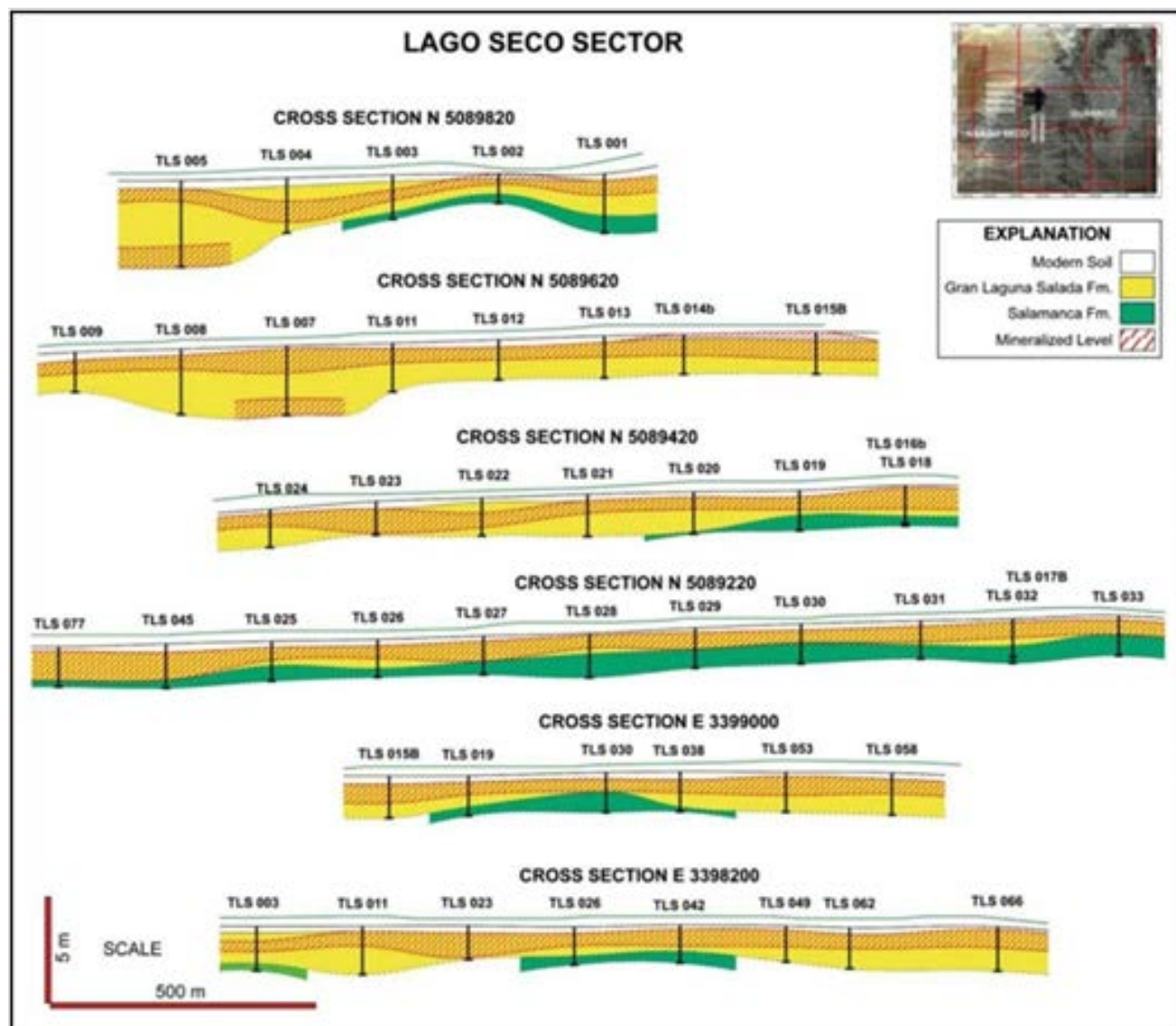
Figure 6-9. Stacked sections showing the distribution of mineralization in the Lago Seco Area. Note the extreme vertical exaggeration (after Inwood and Goode, 2011) (Miller, 2024).
