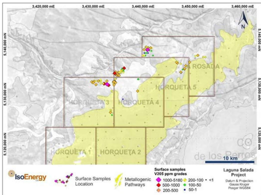
Figure 6-16. La Rosada area of the Laguna Salada Property (historical boundary) showing surface sample locations and V2O5 ppm concentrations (Miller, 2024).
