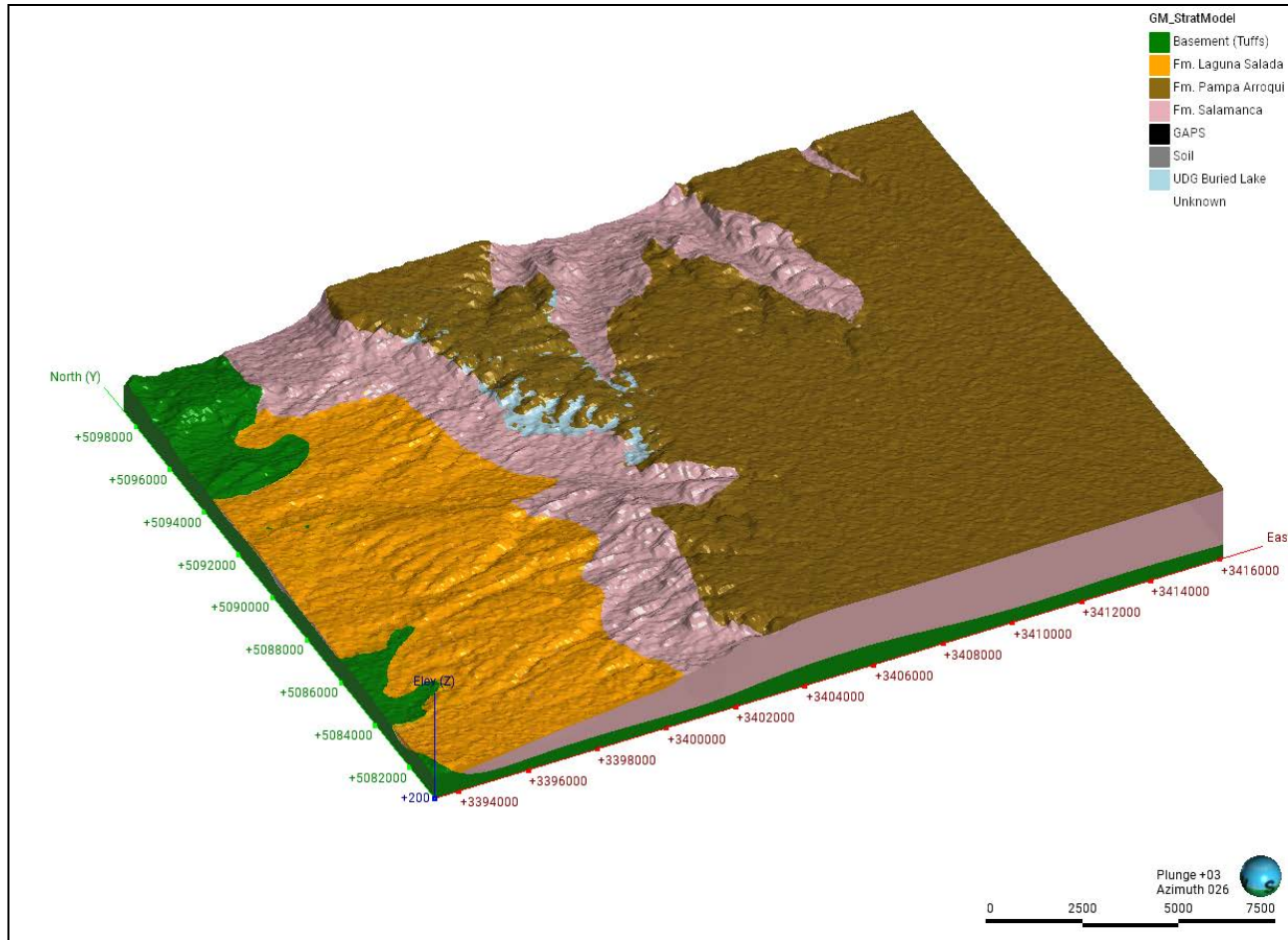
Figure 14-2. Isometric view of the Laguna Salada lithology model looking towards azimuth 026° with plunge +03°, showing the modelled basement/tuff units, Gran Laguna Salada Formation, Pampa de Arroqui Formation, Salamanca Formation and Buried Lake unconformity-related unit. The view is displayed with 10× vertical exaggeration (Z-scale = 10.0) for visualization (Atticus, 2026).
