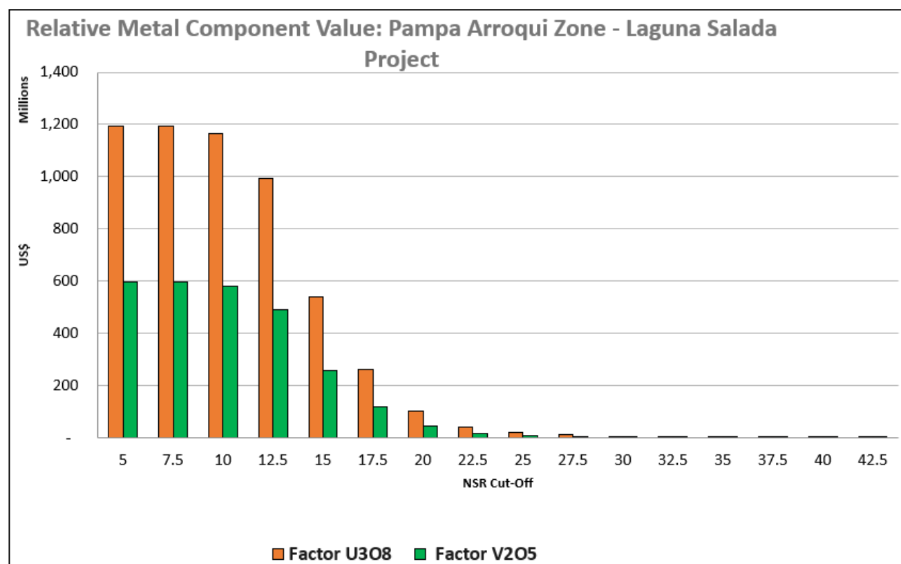
Figure 14-41. Relative metal component value by NSR cut-off for the Pampa de Arroqui domain, showing the relative contribution of U_3O_8 and V_2O_5 to modelled value (Atticus, 2026).
