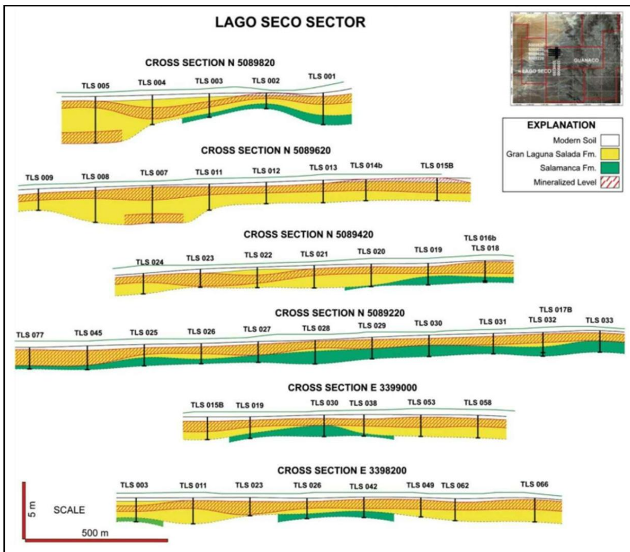
Figure 7-7. Stacked sections showing the distribution of mineralization in the Lago Seco area. Note extreme vertical exaggeration (after Inwood and Goode, 2011; Miller, 2024).
