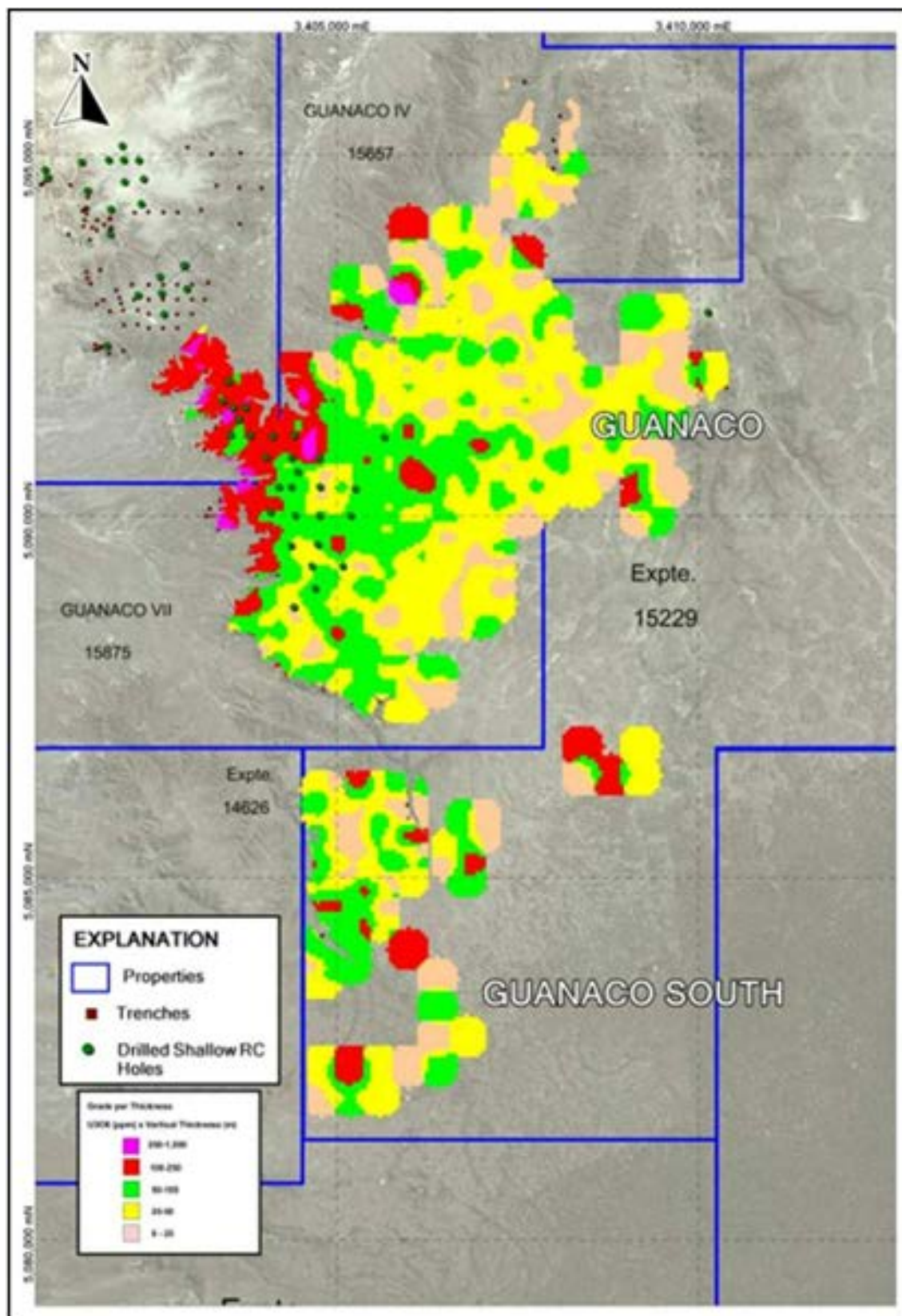
Figure 6-5. Grade-thickness distribution map of the Guanaco Region, U3O8 (ppm) x m (after Inwood and Goode, 2011) (Miller, 2024).
