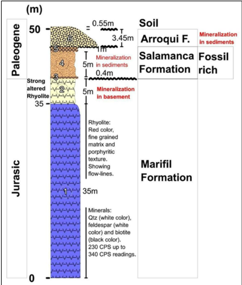
Figure 6-23. Stratigraphic column at La Rosada, Delfin and Pescado prospect areas (Miller, 2024).
