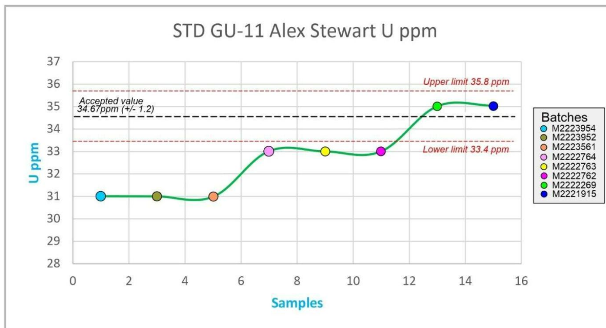
Figure 11-7. Uranium values for ASI internal standard GU-11, certified 34.67 ppm U (Miller, 2024).
