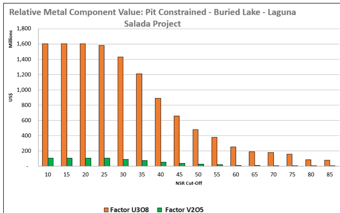
Figure 14-43. Relative metal component value by NSR cut-off for the Buried Lake pit constrained domain, showing the relative contribution of U_3O_8 and V_2O_5 to modelled value (Atticus, 2026).
