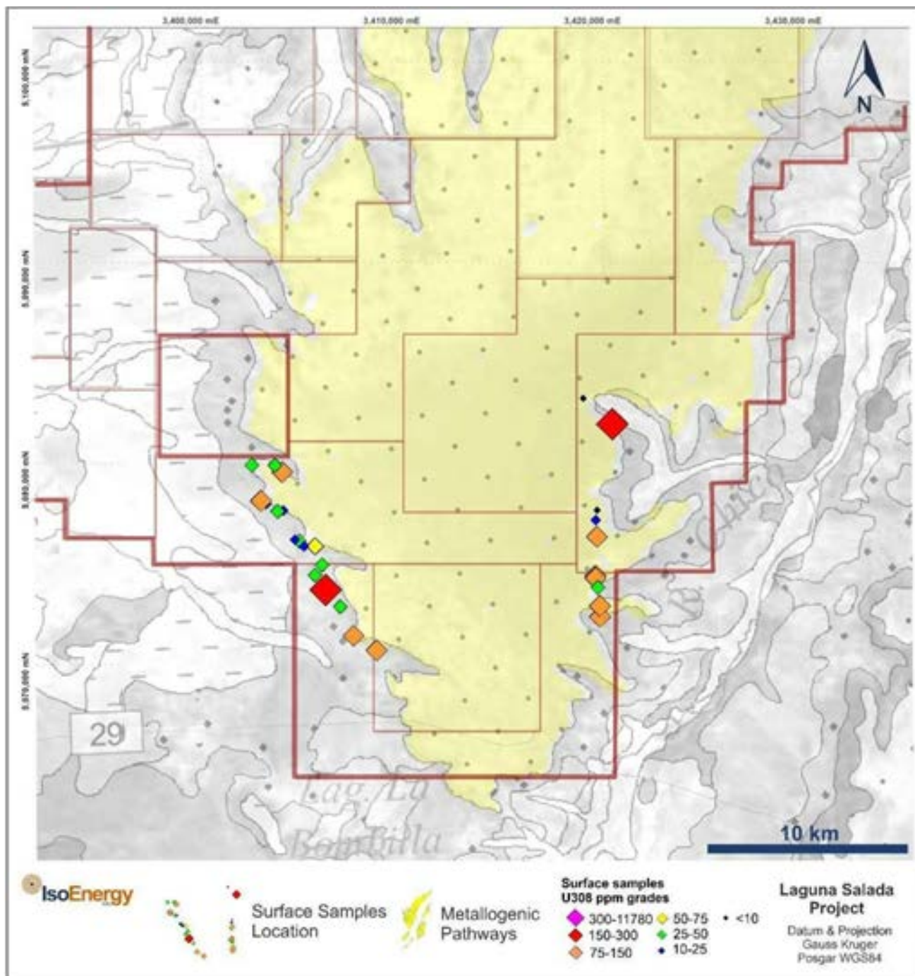
Figure 6-13. La Susana area of the Laguna Salada Property (historical boundary) showing surface sample locations and U3O8 ppm concentrations (Miller, 2024).
