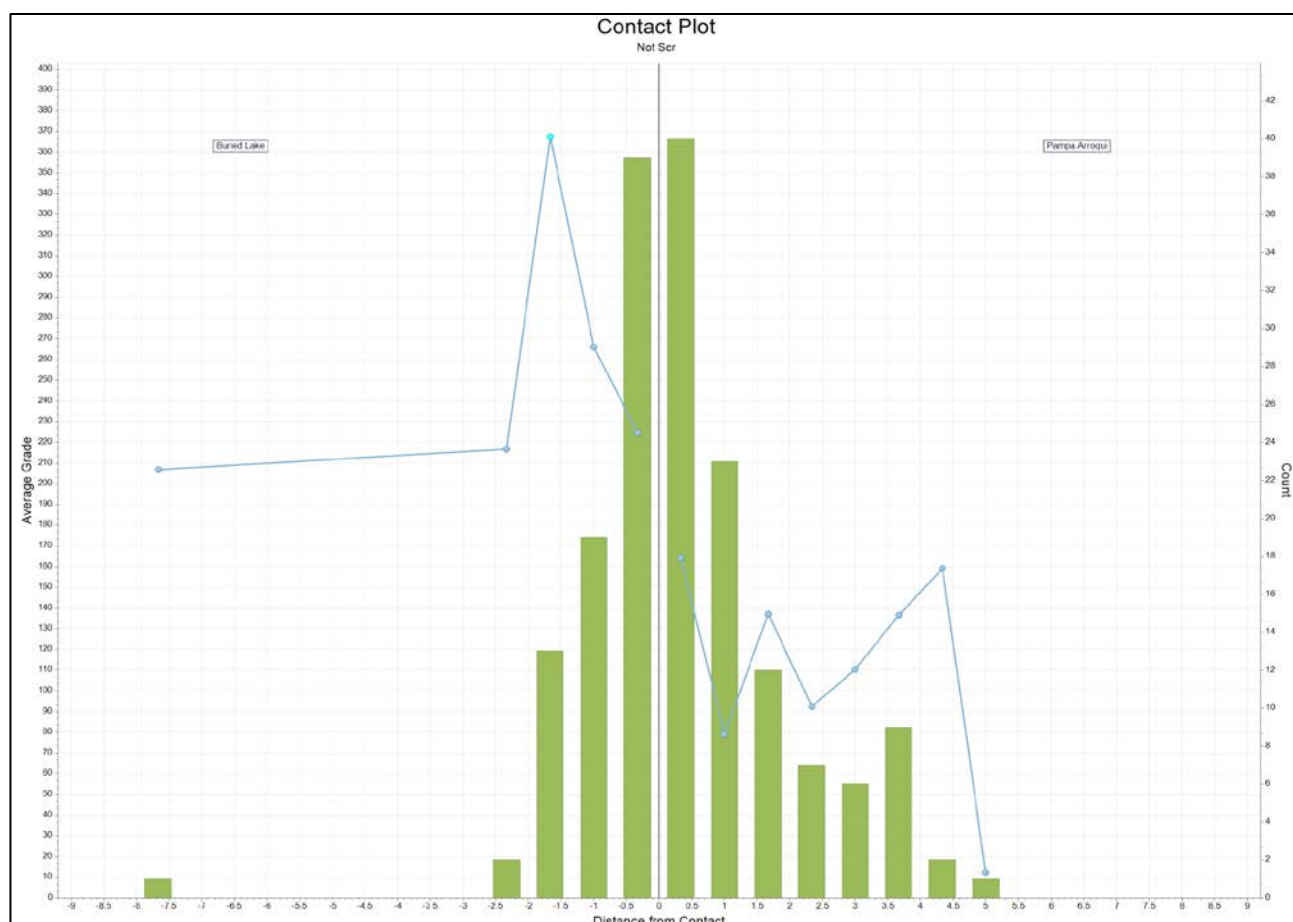
Figure 14-16. Contact plot for unscreened U_3O_8 samples across the Buried Lake to Pampa de Arroqui domain boundary. Negative distances are on the Buried Lake side of the contact and positive distances are on the Pampa de Arroqui side; bars show sample count, and the line shows average grade by distance bin (Atticus, 2026).
