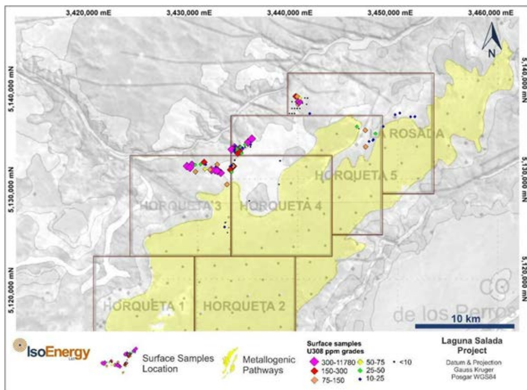
Figure 6-15. La Rosada area of the Laguna Salada Property (historical boundary) showing surface sample locations and U3O8 ppm concentrations (Miller, 2024).
