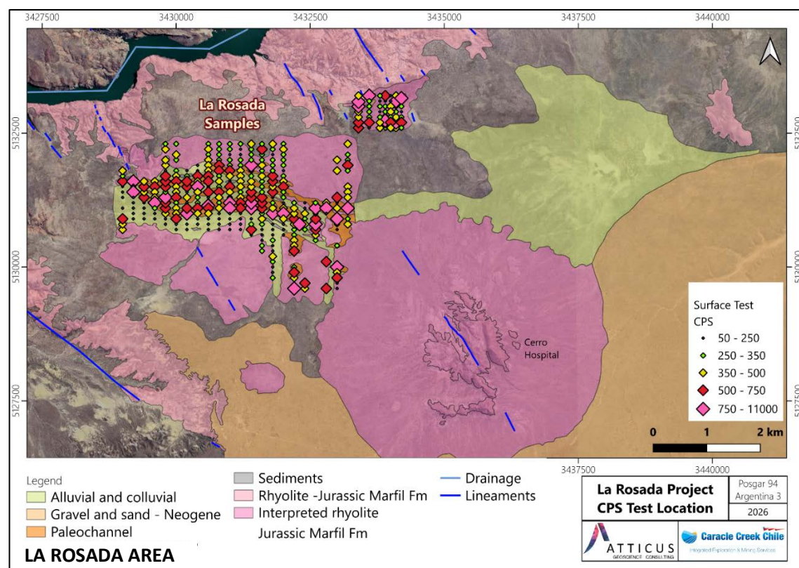
Figure 6-26. Scintillometer readings in counts per second (cps) at La Rosada (Atticus, 2026).
