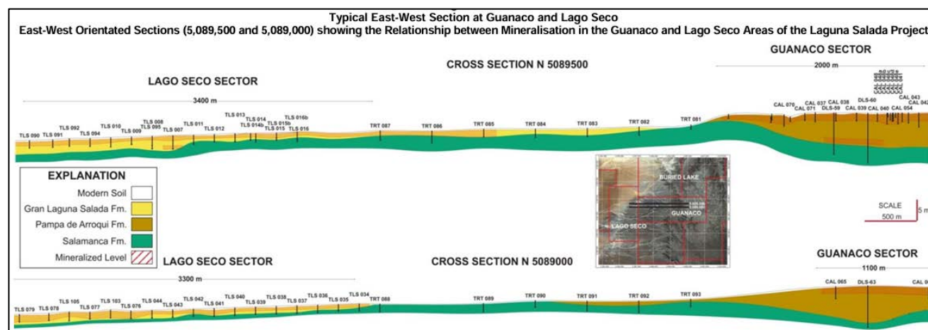
Figure 7-11. Typical east-west sections N 5,089,500 and N 5,089,000 through the Lago Seco and Guanaco sectors, showing the stratigraphic relationship between the Gran Laguna Salada, Pampa de Arroqui and Salamanca formations and the position of the mineralized horizon (Inwood and Goode, 2011).
