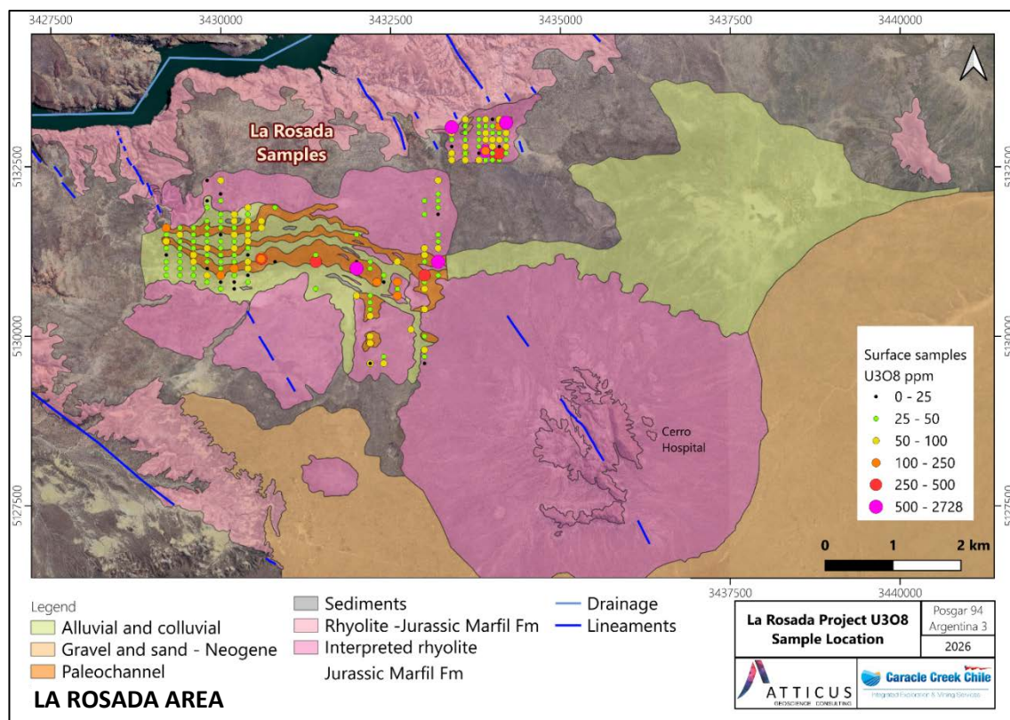
Figure 6-24. Surface sample locations and U3O8 concentrations at the La Rosada area (Miller, 2024).
