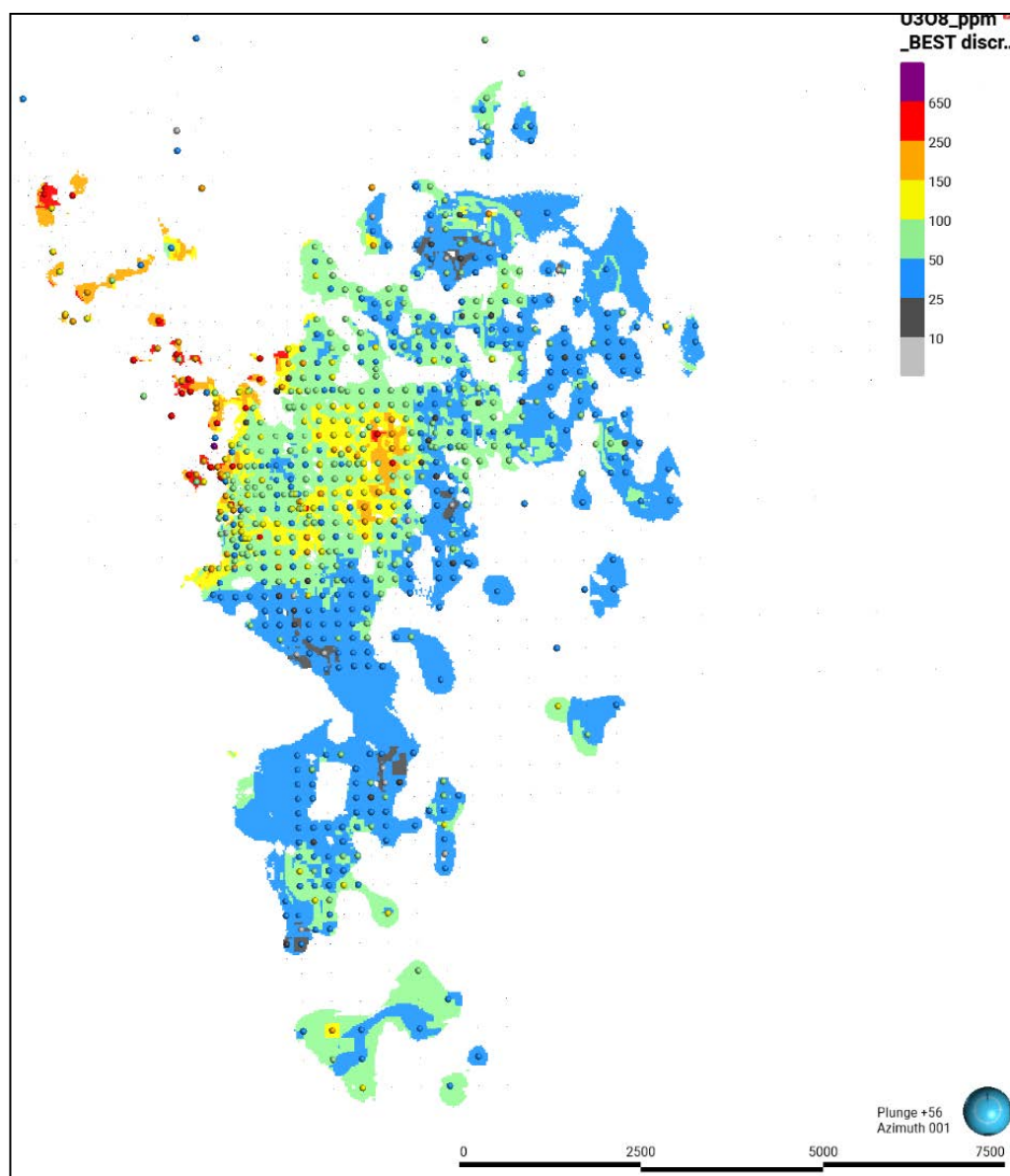
Figure 14-32. Plan view of the Pampa de Arroqui block model showing estimated U_3O_8 block grades with informing U_3O_8 composite grades overlain (Atticus, 2026).
