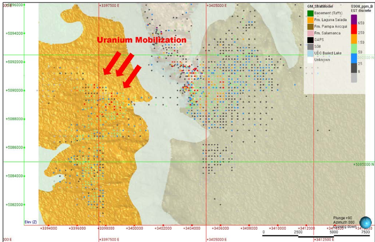
Figure 14-7. Plan view of the Laguna Salada mineralization model showing U_3O_8 grade distribution across the Lago Seco and adjacent Guanaco areas, with interpreted uranium mobilisation direction overlain on the modelled lithological units. (Atticus, 2026).
