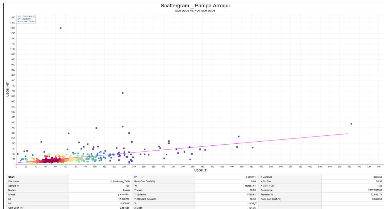
Figure 14-12. Scattergram of screened U_3O_8 versus unscreened U_3O_8 for the Pampa de Arroqui mineralized area. The x-axis represents U_3O_8\_T and the y-axis represents U_3O_8\_NT (Atticus, 2026).
