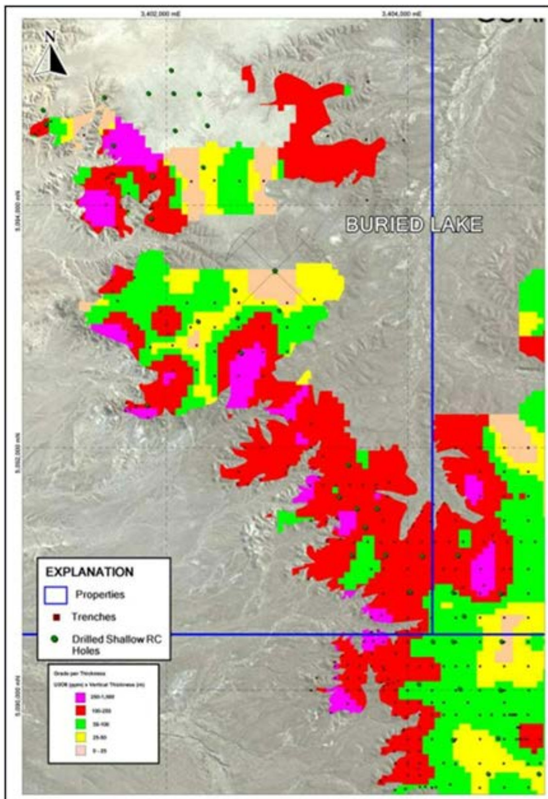
Figure 6-11. Grade-thickness distribution map of the Buried Lake region, U3O8 ppm x metres (after Inwood and Goode, 2011) (Miller, 2024).
