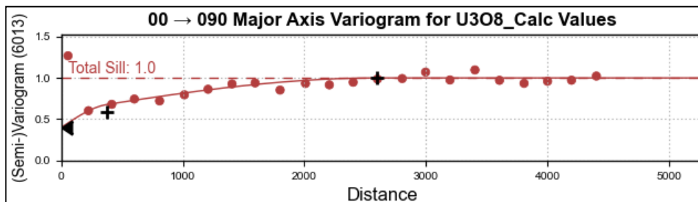
Figure 14-26. Horizontal major-axis variogram for calculated U_3O_8 values in the Pampa de Arroqui estimation domain, showing the fitted model used to support grade-continuity interpretation (Atticus, 2026).
