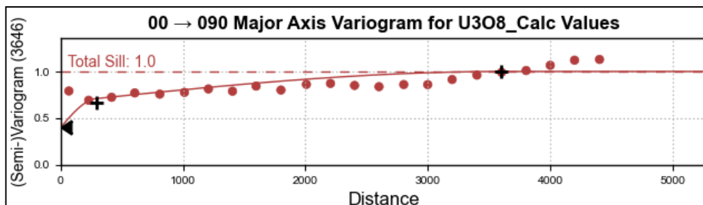
Figure 14-25. Horizontal major-axis variogram for calculated U_3O_8 values in the Laguna Salada estimation domain, showing the fitted model used to support grade-continuity interpretation (Atticus, 2026).
