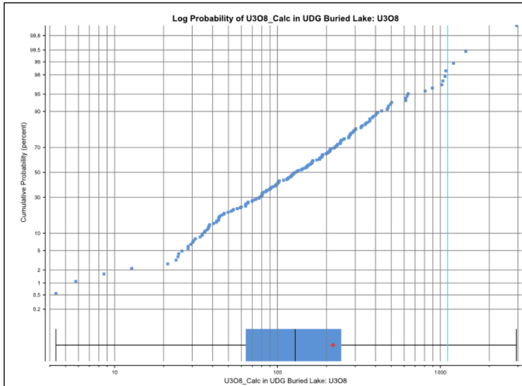
Figure 14-18. Buried Lake U 3 O 8 probability plot showing the upper-tail distribution and selected upper bound applied to the Buried Lake estimation domain (Atticus, 2026).
