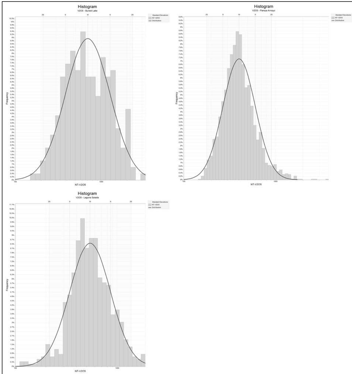
Figure 14-11. V_2O_5 composite histograms for the Laguna Salada, Pampa de Arroqui and Buried Lake mineralized areas. The histograms show vanadium grade distributions used to review grade variability and support separate estimation of V_2O_5 within the area-based estimation domains (Atticus, 2026).
