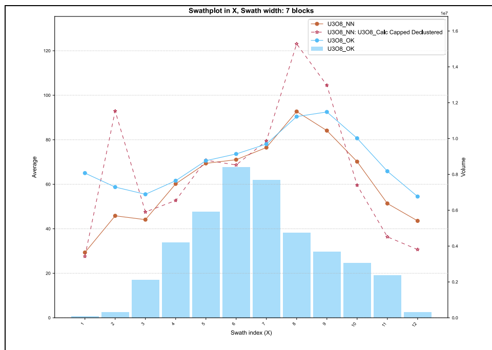
Figure 14-35. Laguna Salada U_3O_8 swath plot validation in the X direction, comparing OK, NN and capped/declustered composite trends with block volume by swath (Atticus, 2026).
