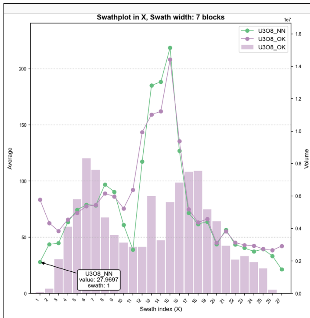
Figure 14-33. Global U_3O_8 swath plot validation in the X direction, comparing OK and NN estimates with block volume by swath (Atticus, 2026).
