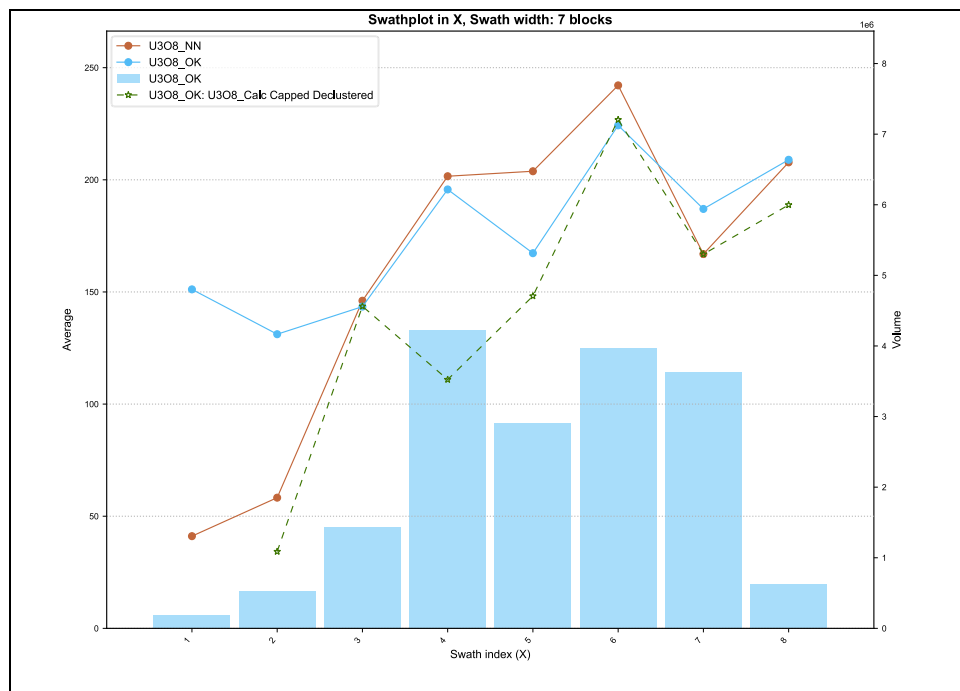
Figure 14-34. Buried Lake U_3O_8 swath plot validation in the X direction, comparing OK, NN and capped/declustered composite trends with block volume by swath (Atticus, 2026).
