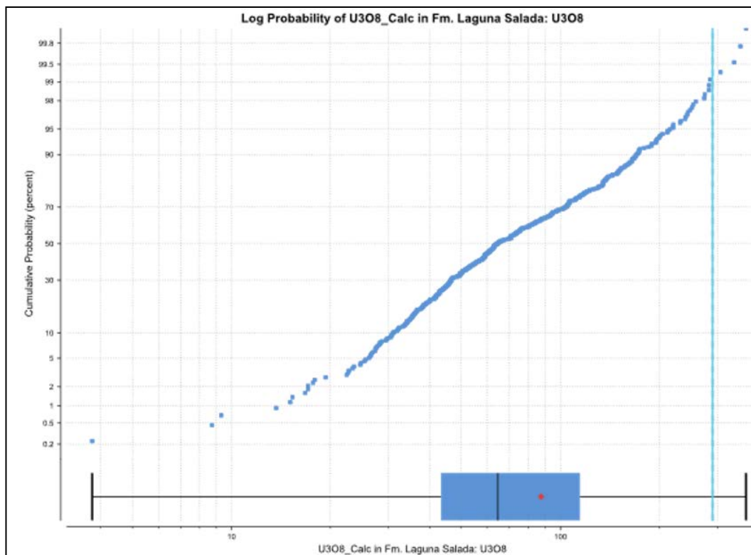
Figure 14-19. Laguna Salada U_3O_8 probability plot showing the upper-tail distribution and selected upper bound applied to the Laguna Salada estimation domain (Atticus, 2026).
